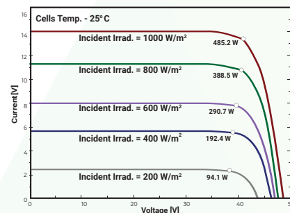
I-V Curve of 535 W at 25°C cell temp and different Irradiance level
